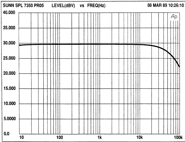
Figure 1. Level vs Frequency into 8 ohms. Input level is 0dBu.
