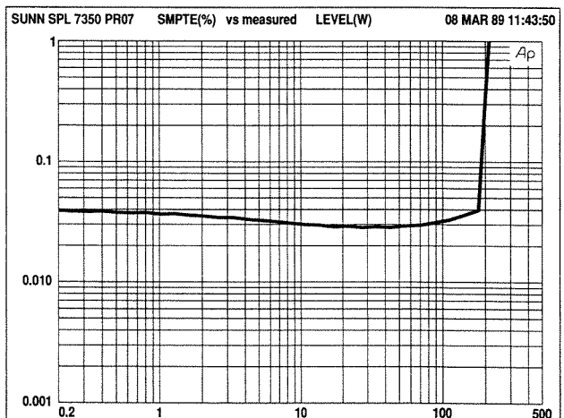
Figure 6. SMPTE IM Distortion vs Output Power into 8 ohms.
