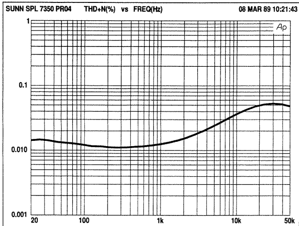
Figure 3. THD vs Frequency at 350 watts into 4 ohms.
