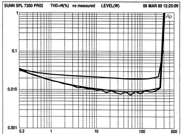
Figure 4. THD vs Output Power into 8 ohms at 20Hz, 2kHz, & 20kHz.
