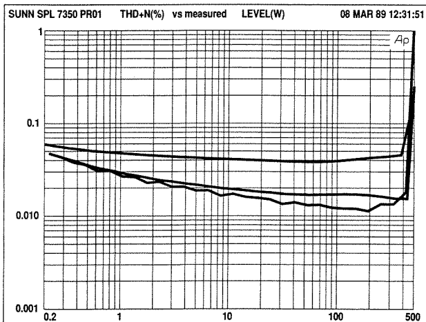
Figure 5. THD vs Output Power into 4 ohms at 20Hz, 2kHz, & 20kHz.
