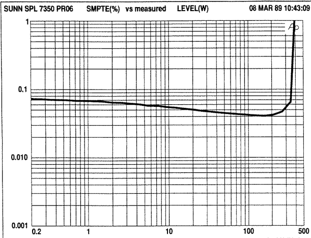
Figure 7. SMPTE IM Distortion vs Output Power into 4 ohms.
