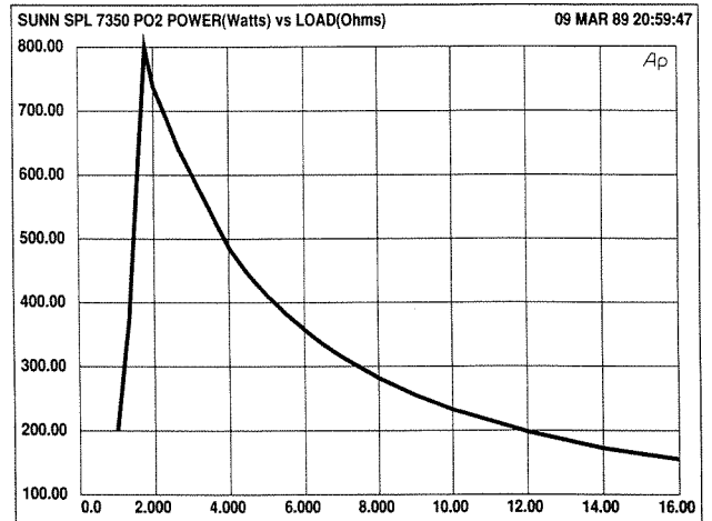
Figure 10. Single Channel Output Power vs Load Impedance at 1kHz.
