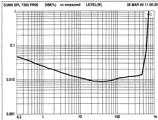
Figure 9. DIM100 Distortion vs Output Power into 4 ohms.
