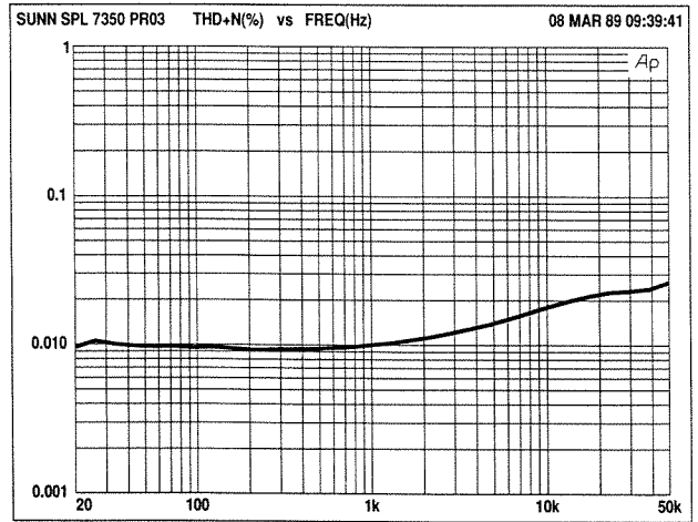
Figure 2. THD vs Frequency at 200 watts into 8 ohms.
