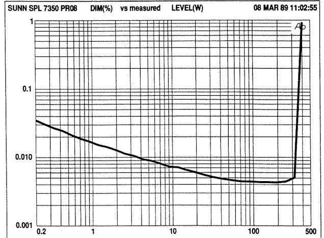
Figure 8. DIM100 Distortion vs Output Power into 8 ohms.
