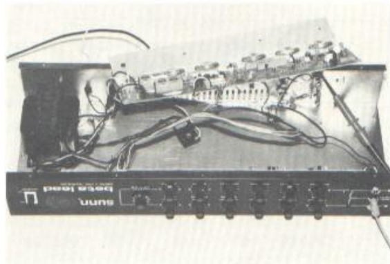
Pre-amp Servicing – Diagram Two
