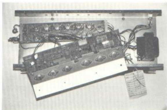
Pre-amp Disassembly – Diagram Three
