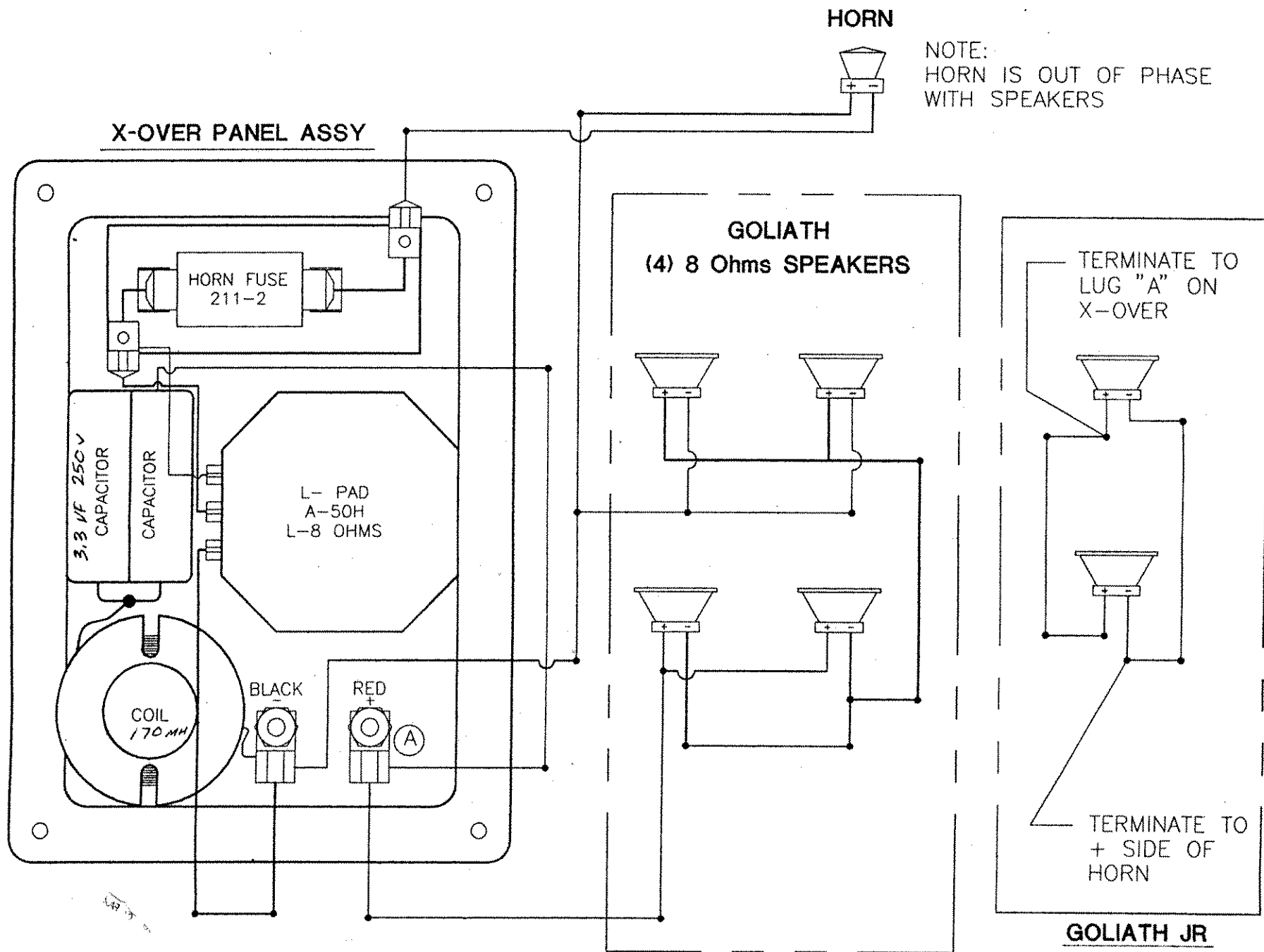
OLD STYLE X-OVER LAYOUT
